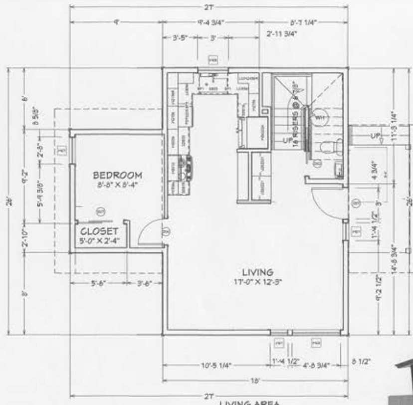
1st Floor 1/4 in = 1 ft
