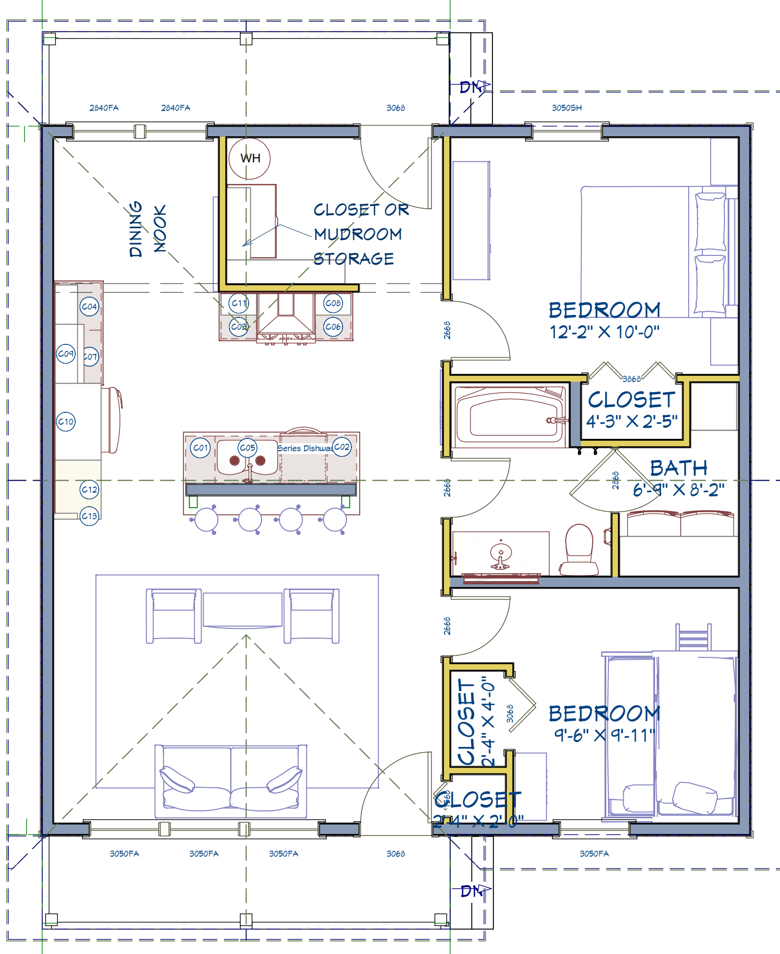
1st Floor 1/4 in = 1 ft
